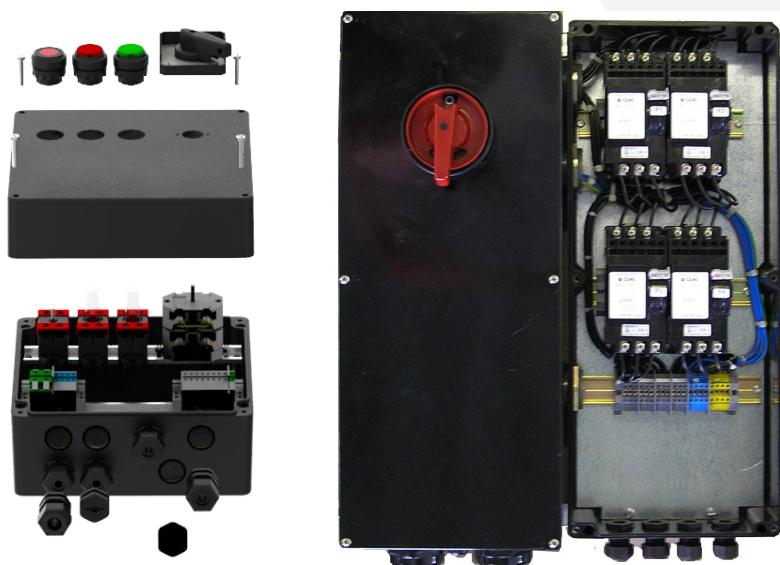
Example: Ex control units with GRP enclosures
