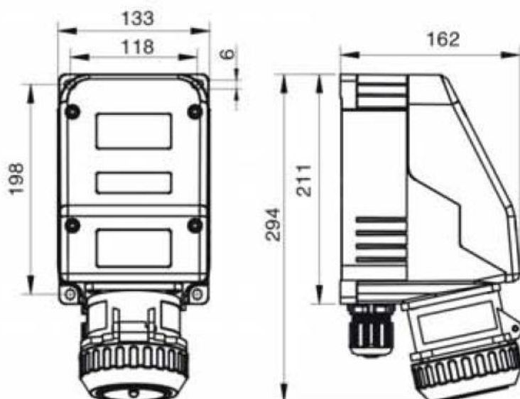
WALL SOCKET (all dimension in mm)
