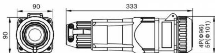
COUPLER SOCKET (all dimension in mm)
