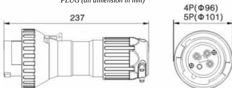
PLUG (all dimension in mm)
