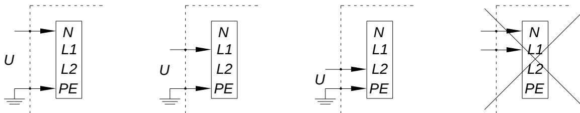
Wiring diagram
